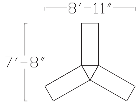
Y Configuration Plan Overall Dimensions as shown
